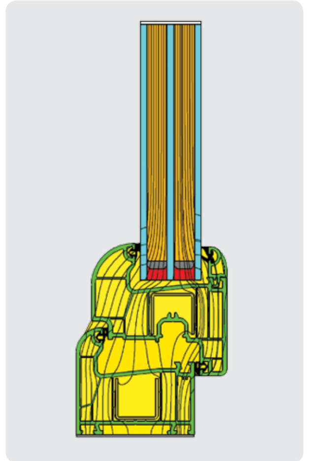
PENCERE ISI AKIŞ DİYAGRAMI UF: 1,2 W/M 2 *K UW: 1,05 W/M 2 *K
